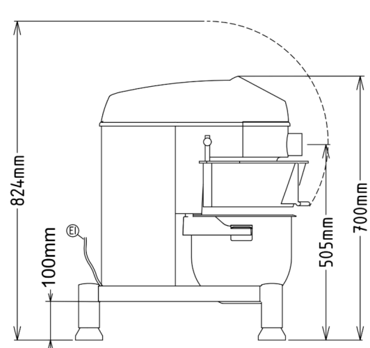
Side
